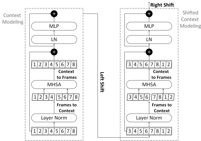
Fig. 2. Swin transformer for speech with 8 frame tokens.
