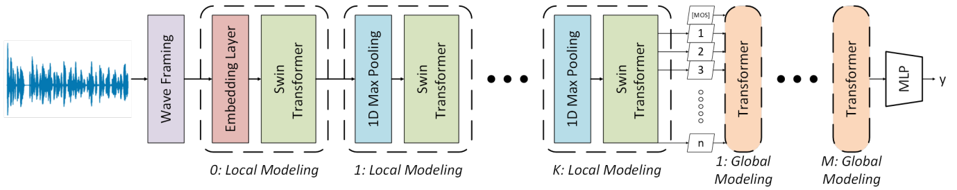
Fig. 1. The architectural diagram of our proposed SWIM model. y corresponds to the MOS prediction of the input utterance.
